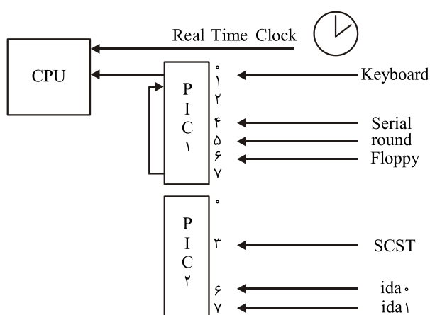
Figure: A Logical Diagram of Interrupt Routing
